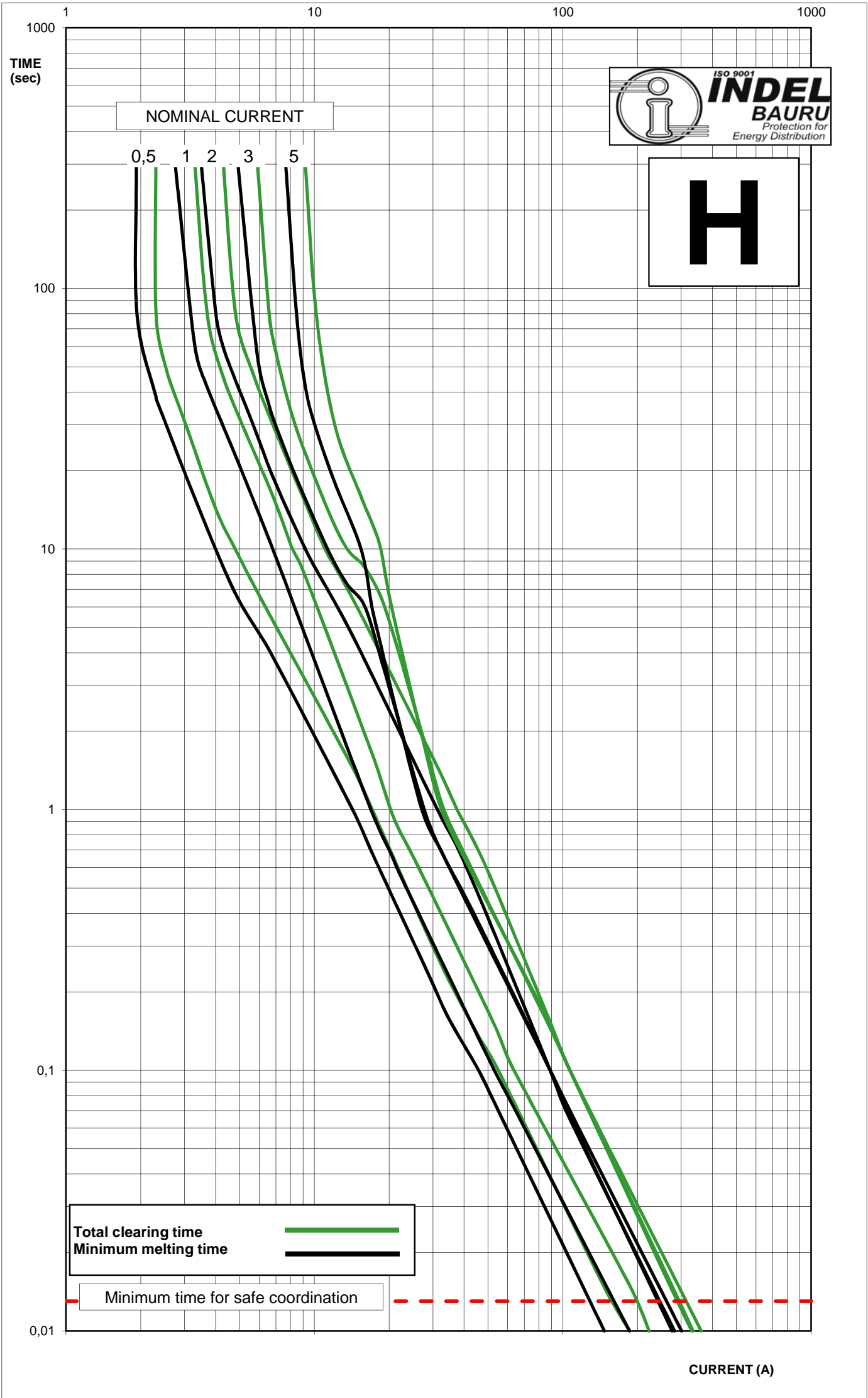
CHARACTERISTICS CURVES FUSION TIME x CURRENT TYPE "H" - COMPLY WITH STANDARD NBR 5359 DATE: 09/02
