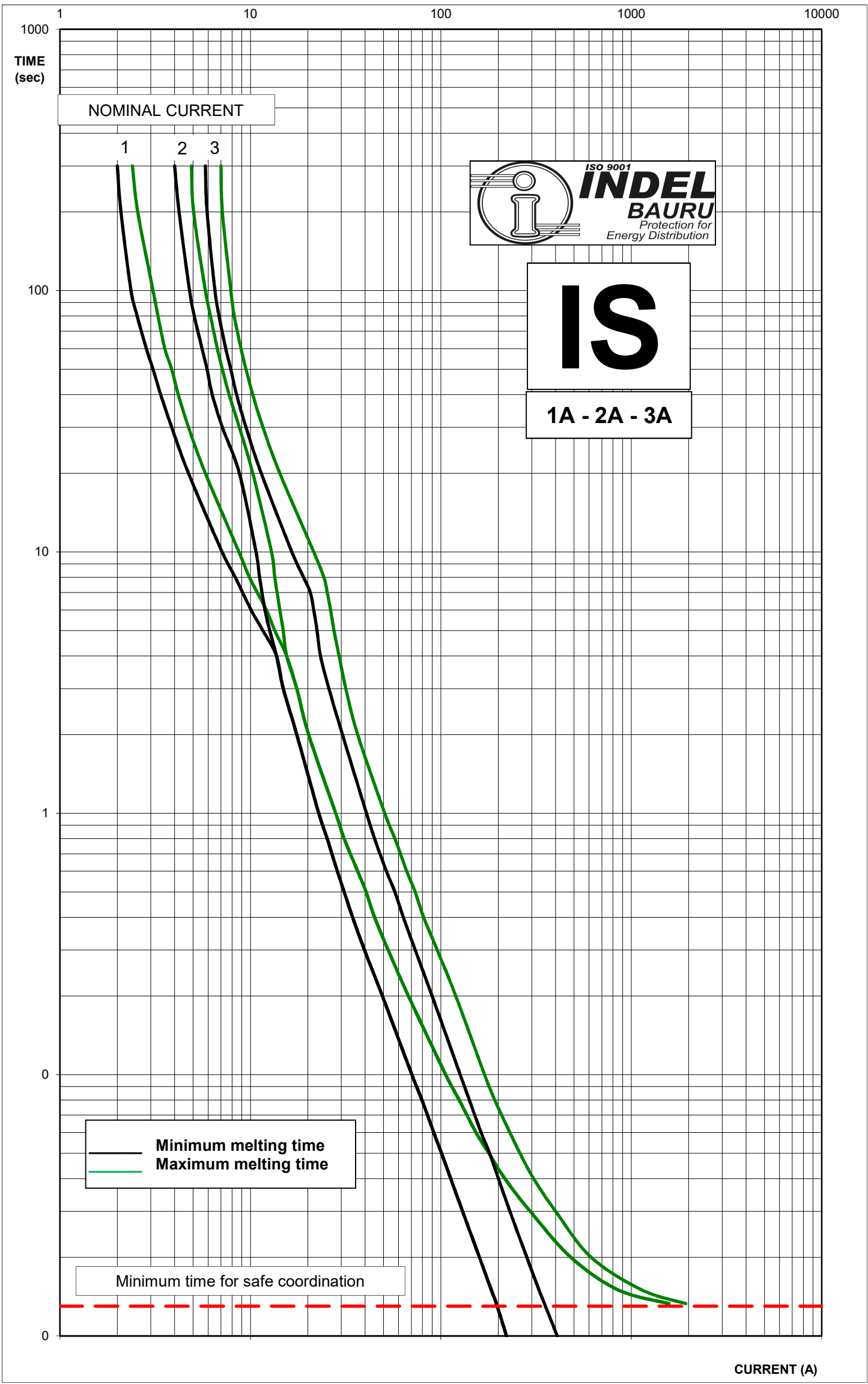
CHARACTERISTICS CURVES FUSION TIME x CURRENT TYPE "IS" - COMPLY WITH STANDARD ANSI C34.42-1996 DATE: 02/18
