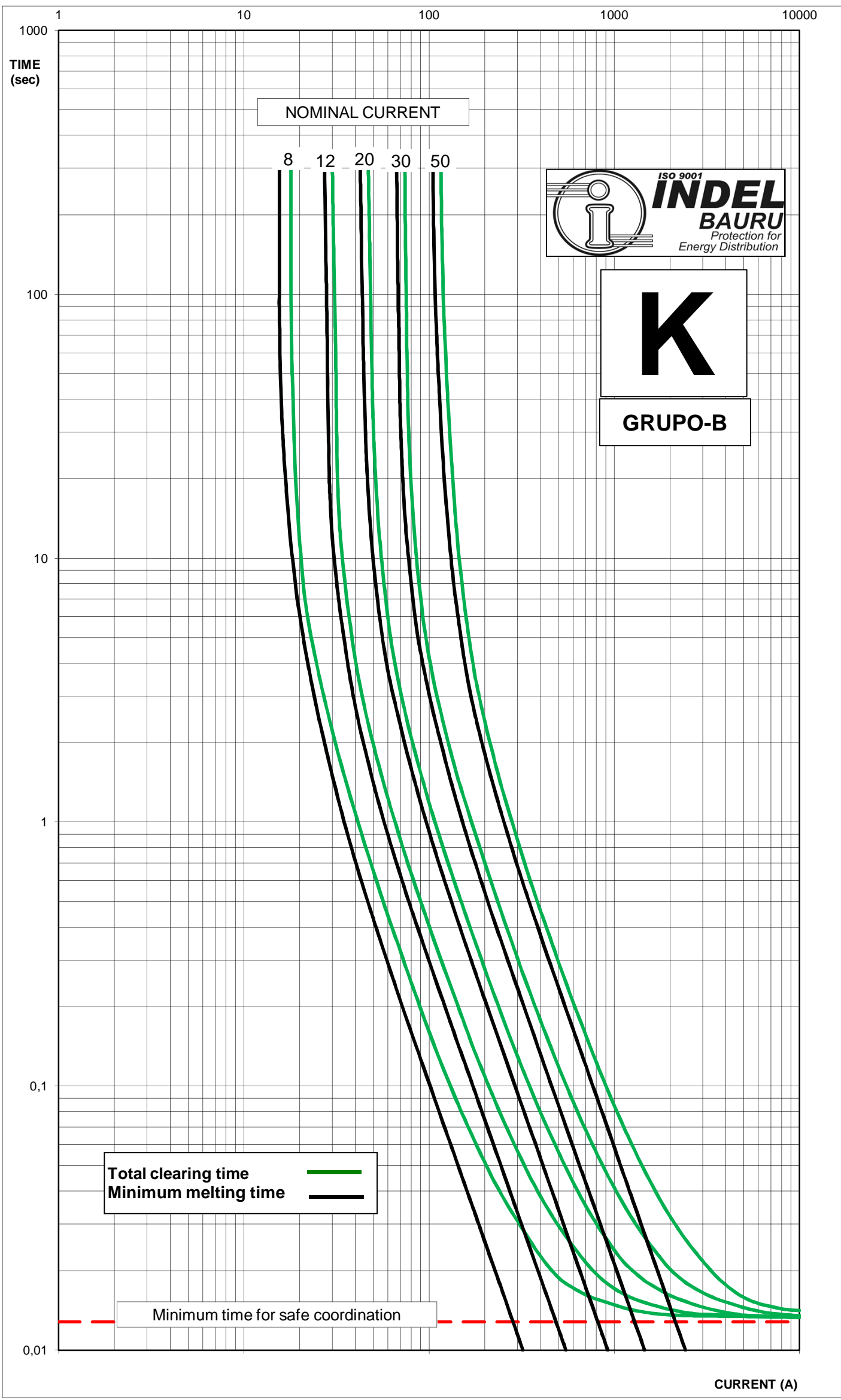
CHARACTERISTICS CURVES FUSION TIME x CURRENT TYPE "K OPEN" - COMPLY WITH STANDARD ANSI C37.42-1996 DATE: 09/02
