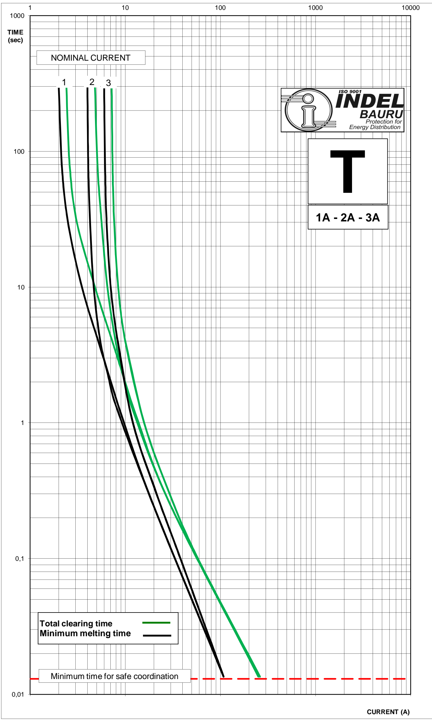
CHARACTERISTICS CURVES FUSION TIME x CURRENT TYPE "T OPEN" - COMPLY WITH STANDARD ANSI C37.42-1996 DATE: 09/02
